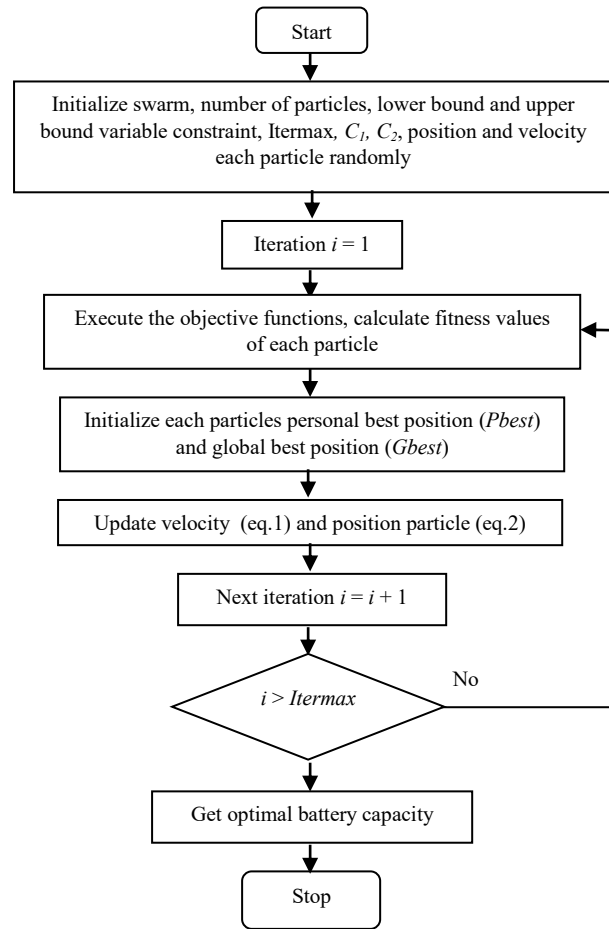
Fig. 3. Flow Chart of the PSO Algorithm
